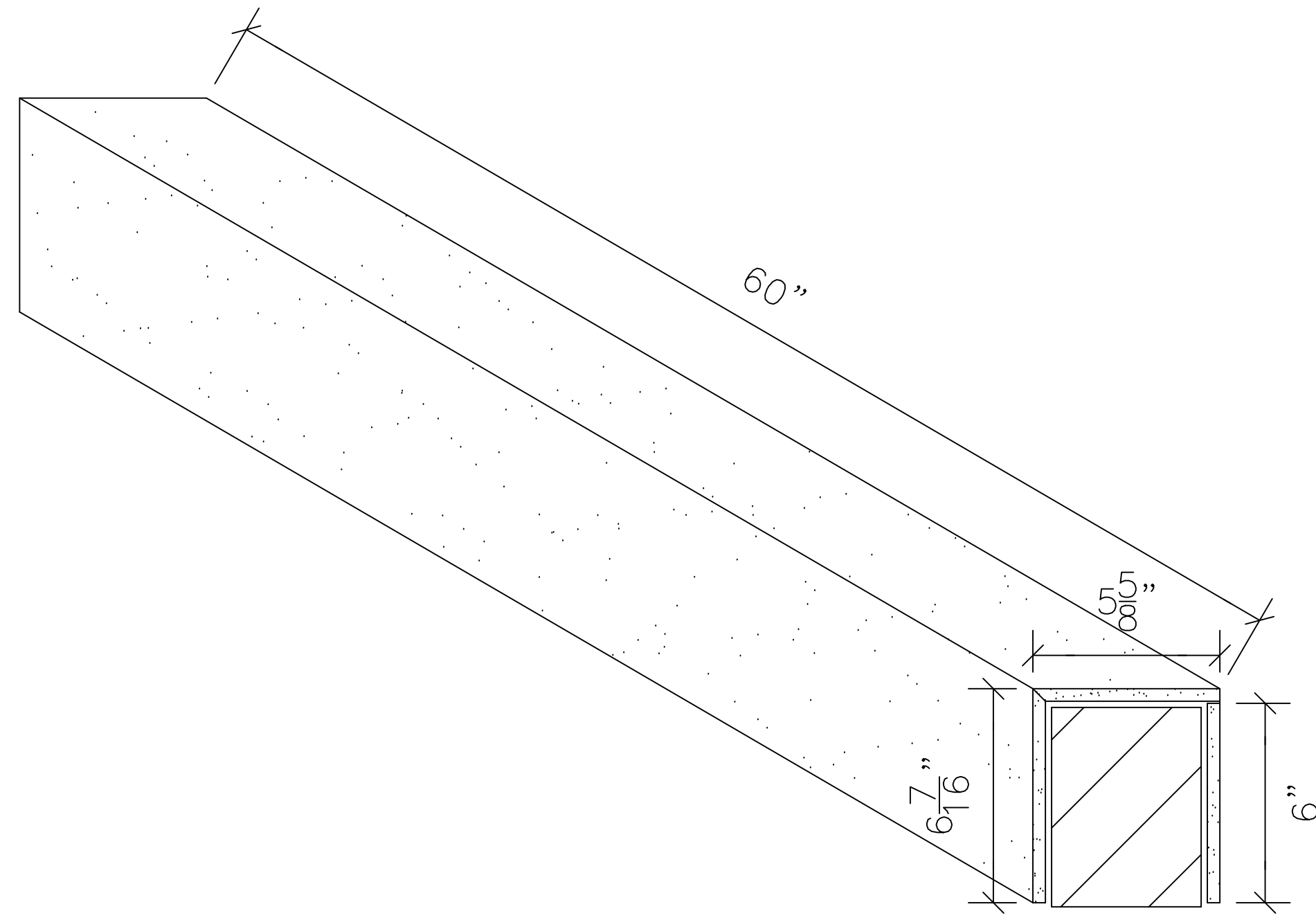
SHOWER CURB Scale: NTS
